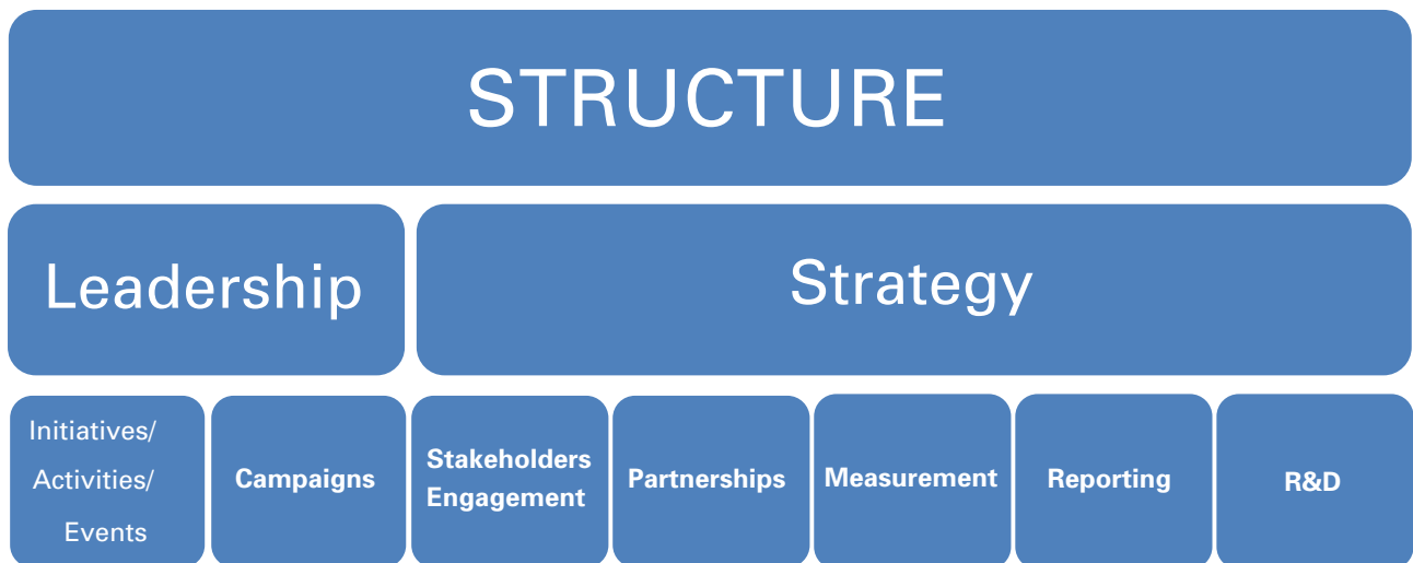
Figure 1 | Sustainability Model
